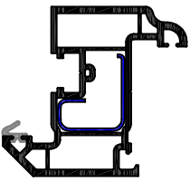
P104 70mm Externally Beaded Chambered Glazing Bead R103 Shell Sash Reinforcement
