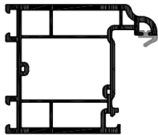
P118 (with PCE) / P218 (with PCE) 82mm Outer Frame
