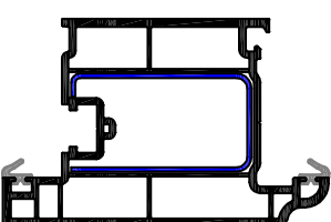
P219 (with PCE) 110mm Internal Beaded outward Opening Door Sash Shell Door Sash Reinforcement
