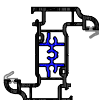
P106 (with PCE) 70mm Z-Trim / Mullion A113 Paked Aluminium Reinforcement
