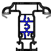
P102 (with PCE) / P202 (with PCE) 70mm T-Trim A113 Paked Aluminium Reinforcement
