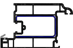
P105 110mm Externally Beaded outward Opening Door Sash Shell Door Sash Reinforcement
