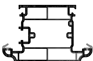
P222 (with PCE) 110mm Door Sash / Mullion
