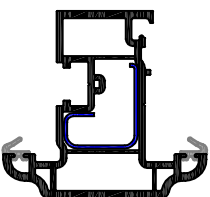
P217 (with PCE) Internal Bead Reinforcement Sash R103 Shell Sash Reinforcement
