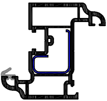
P103 70mm Externally Beaded Chambered Glazing Bead R103 Shell Sash Reinforcement
