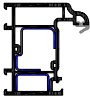
P101 (with PCE) / P201 (with PCE) 80mm Outer Frame R101 Outer Frame Steel Reinforcement Shell High Reinforcement
